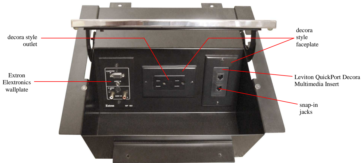
inside of power box
