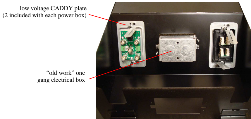
backside of power box
